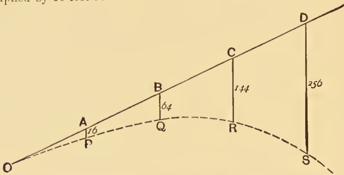
FIG. 35.—Curve described by a projectile, showing how it drops from the line of fire, OD , in successive seconds, the same distances, AP , BQ , CR , &c., as are stated above for a dropped body ( cf. p. 170).
